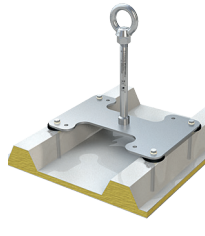
ABS-Lock® X-SW
