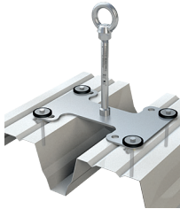
ABS-Lock® X-T-21
